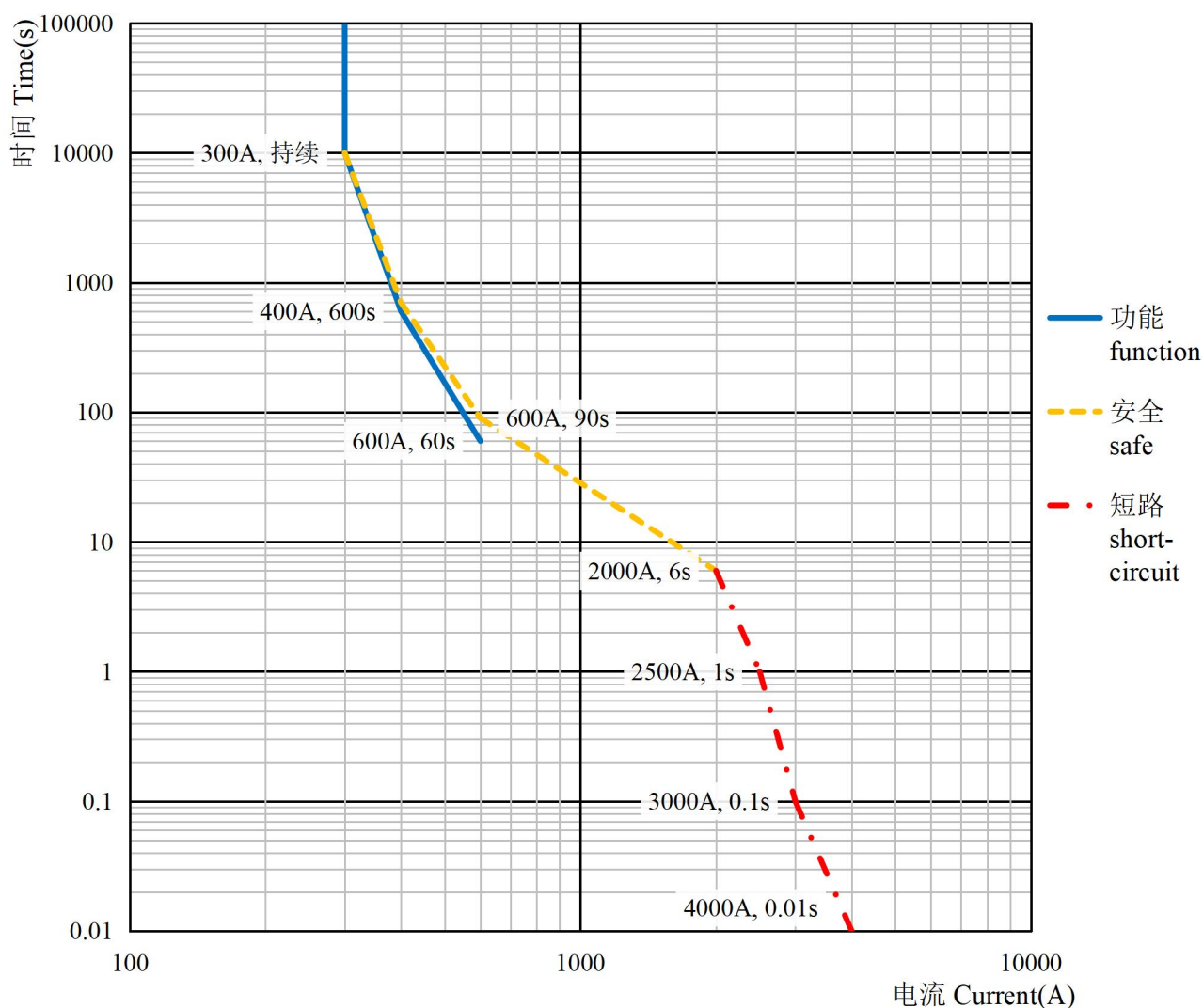
电流耐受曲线 Current Endurance Curve
